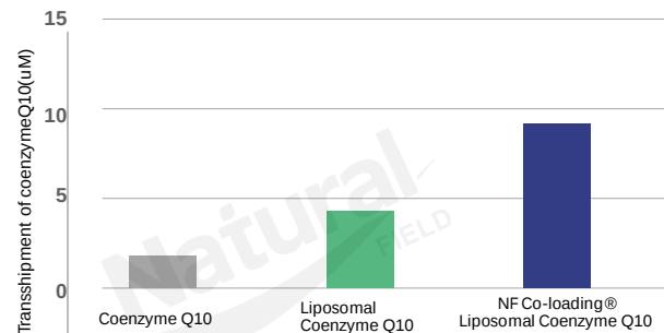
Relative Absorption
